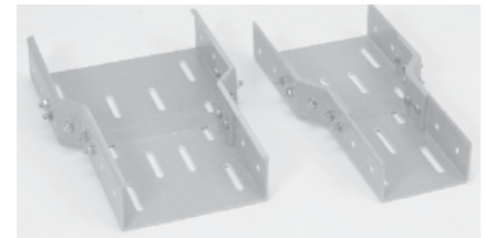
Straight Reducer
