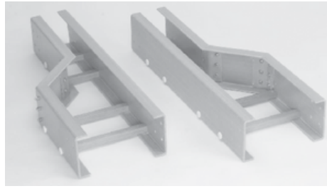
Right Hand Reducer
