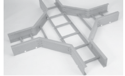
90° Horizontal Cross
